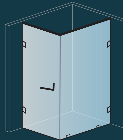
ONE FIXED GLASS & ONE DOOR (HINGES ON WALL)
