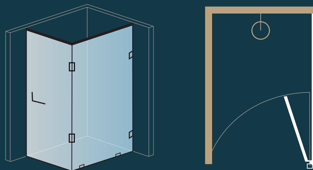
ONE FIXED GLASS & ONE DOOR (HINGES ON GLASS CORNER)
